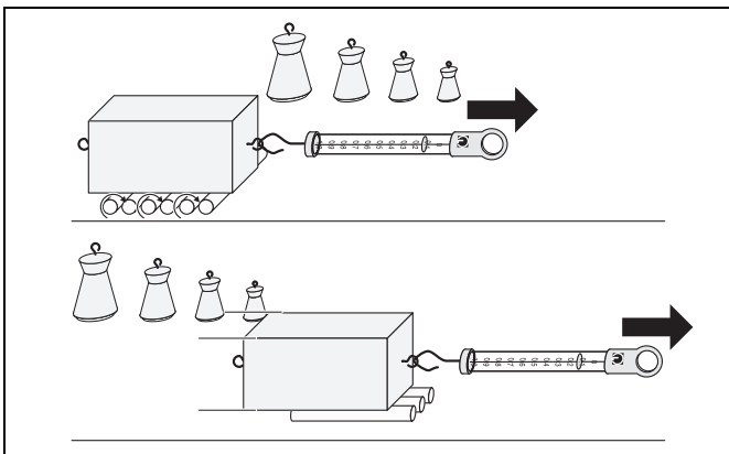
Fig. 3 Measuring the rolling friction force F_R (top) and the sliding friction force F_G (bottom) as a function of the force of gravity G .
