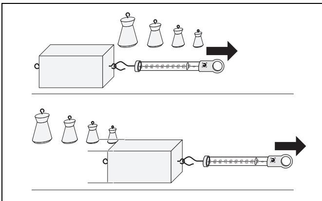
Fig. 2 Measuring the static friction force F_H (top) and the sliding friction force F_G (bottom) as a function of the force of gravity G .
